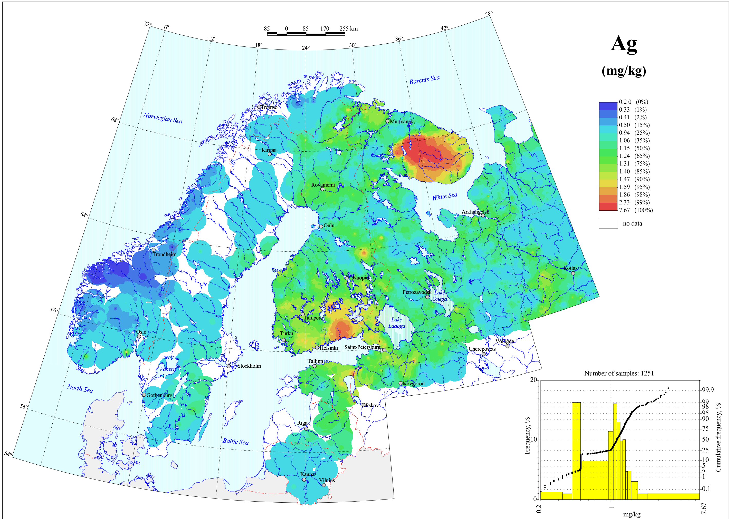
Silver in C-horizon, Grain Size <2 mm, Total Content
